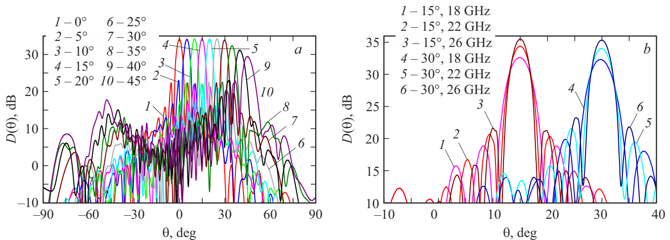
Figure 3. Calculated antenna patterns in the E plane at frequency F = 22 GHz with different angles of BFN rotation ( a ) and at various frequencies with two BFN positions ( \varphi = 15^\circ, 30^\circ ) ( b ). A color version of the figure is provided in the online version of the paper.
