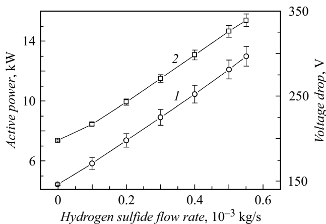
Figure 2. Dependences of voltage drop (1) and active power (2) of the plasma torch on the mass flow rate of hydrogen sulfide; the argon flow rate in the electrode zone is 3 \cdot 10^{-3} kg/s, the argon flow rate in the arcing zone is 3 \cdot 10^{-3} kg/s, and the average effective current value is 31.8 A.
