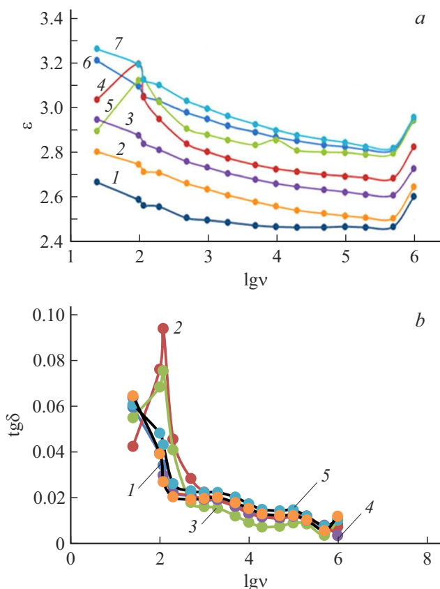
Figure 3. Frequency dependences \varepsilon = f(\nu) and \text{tg } \delta = f(\nu) for the PP+Na + (MMT) composite irradiated with a dose of 100 kGy at temperature T = 298 K. Na + (MMT), vol.%: a ) 1 — 2, 2 — 3, 3 — 5, 4 — 6, 5 — 7, 6 — 0.5, 7 — 0; b ) 1 — 0, 2 — 0.5, 3 — 7, 4 — 5, 5 — 2.
