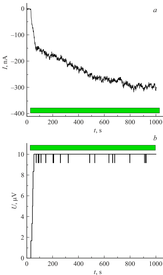
Figure 2. Generation of current (a) and open-circuit EMF (b) in the Pd/PdH system. The colored area indicates that the structure is in the hydrogen atmosphere.
