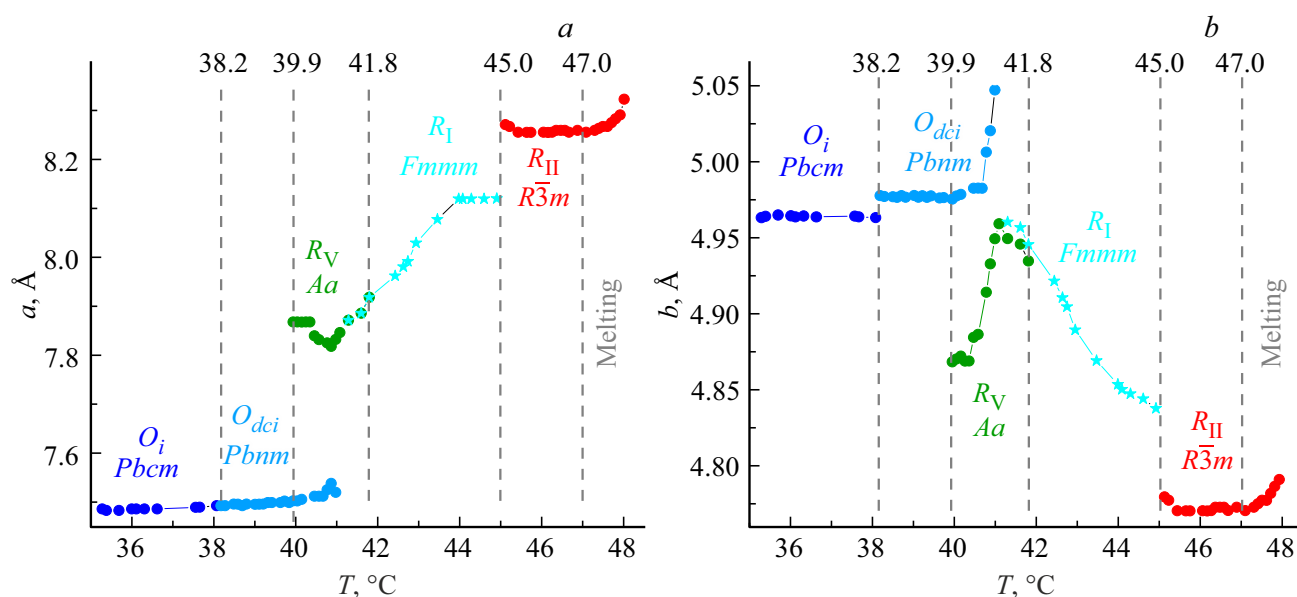
Figure 7. Temperature changes of the parameters a (a) and b (b) of the lattice cells of polymorphic modifications of tricosane in case of heating in the temperature range of \Delta T = 35.0\text{--}48.0^\circ\text{C} .
