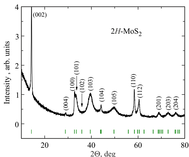
Figure 1. Diffraction pattern of original compound MoS 2 . The lower dashes indicate the positions of the Bragg reflections for the hexagonal modification of 2H-MoS 2 according to the International Database (Card Number 00-037-1492) [17].
