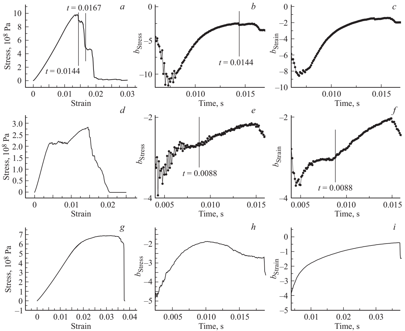
Figure 2. Loading diagram, time dependence of scaling coefficient for stresses ( b_{\text{stress}} ) and strains ( b_{\text{strain}} ) for the sample with orthoclase bonds 48695 d \leq 0.6 (a–c), for the sample with glass bonds (d–f) and for the sample with low-modulus bonds (g–i).
