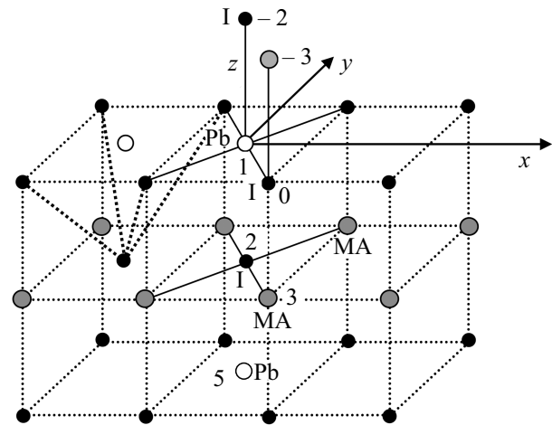
Figure 4. Designations of atoms in the perovskite lattice cell. White circles — Pb atoms, black circles — halogen atoms (atoms 0, 2), gray circles — MA atoms. Halogen tetrahedron edges are shown in the left upper corner.
