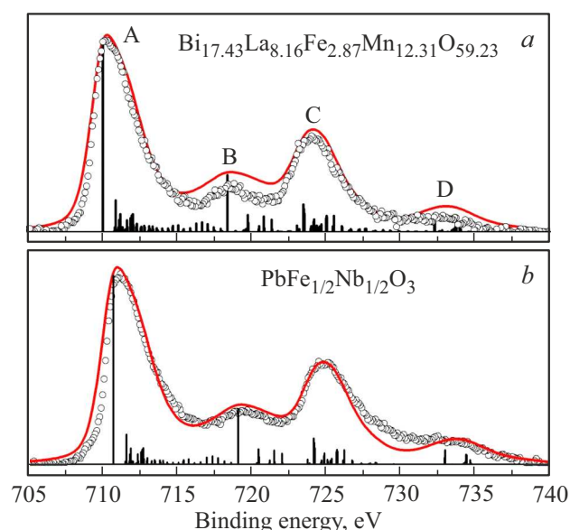
Figure 5. Fe2 p -level spectra for Bi 17.43 La 8.16 Fe 2.87 Mn 12.31 O 59.23 composite compound and single crystal of PbFe 1/2 Nb 1/2 O 3 . Experimental data are shown by circles, calculated data for Fe 3+ ion are shown by columns and a solid line [12].
