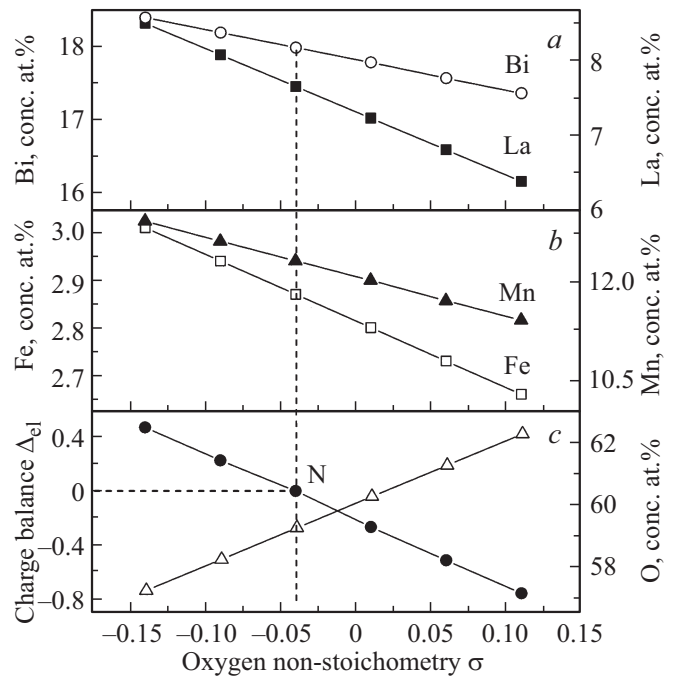
Figure 2. Element concentrations calculated for the sample of Bi 1-x La x Fe 1-y Mn y O 3+σ and the total charge \Delta_{\text{el}} of all ions in the structural unit of the compound at different values of the nonstoichiometry parameter \sigma . The concentrations of elements in the sample were determined with \Delta_{\text{el}} = 0 . The corresponding nonstoichiometry parameter \sigma = -0.04 .
