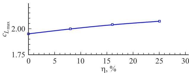
Figure 2. Maximal lift coefficient of the flap profile versus percentage of water vapor in the air.
