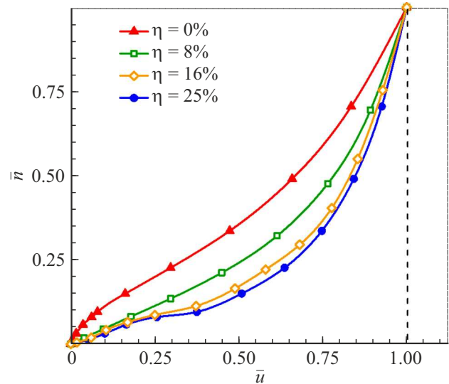
Figure 3. Velocities distribution in the boundary layer in the point on the flap upper surface x = 0.92b
