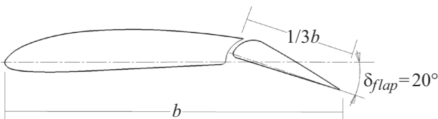
Figure 1. Computational model of the wing-flap profile .
