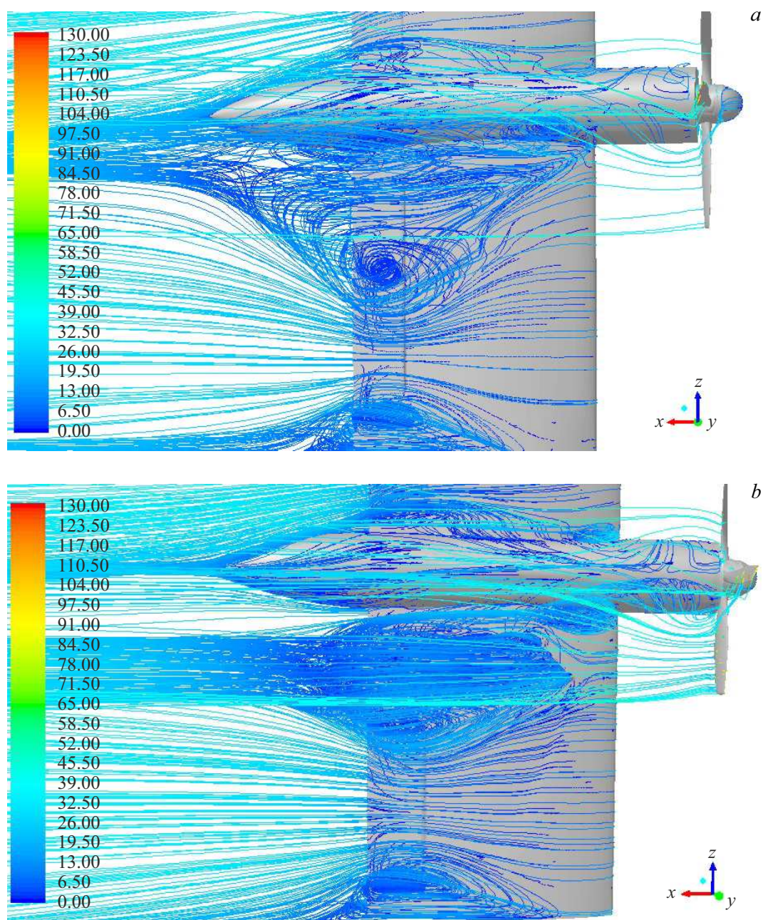
Figure 3. Cross-sectional velocities profile in the middle of the vortex generator: a — without vortex generator, b — with vortex generator.
