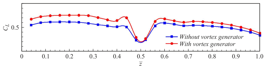
Figure 2. Distribution of the lift coefficient in wing sections.
