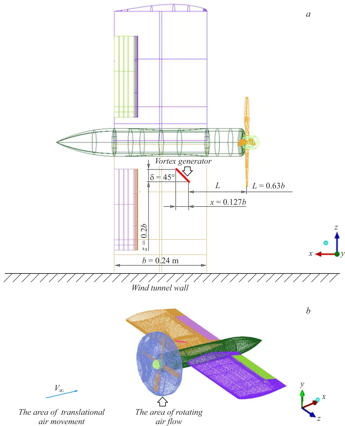
Figure 1. Computational wing model: a — general view, b — building of a computational grid.
