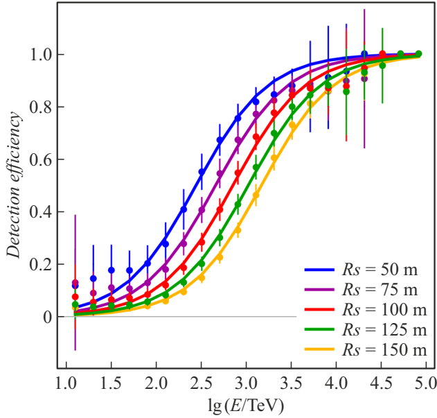
Figure 2. Mean efficiency of joint EAS detection by individual Tunka-Grande installations with different R_s .
