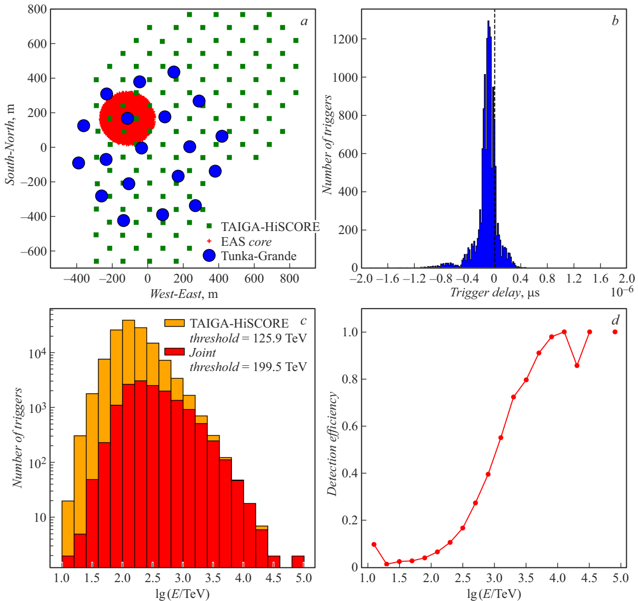
Figure 1. Example of joint events of one of the Tunka-Grande installations and TAIGA-HiSCORE optical detectors: a — layout of installations, optical detectors and EAS axes with event sampling radius R_s = 150 m; b — EAS detection time difference histogram; c — number of EAS's according to the TAIGA-HiSCORE data and joint events depending on the PCR energy; d — joint detection efficiency.
