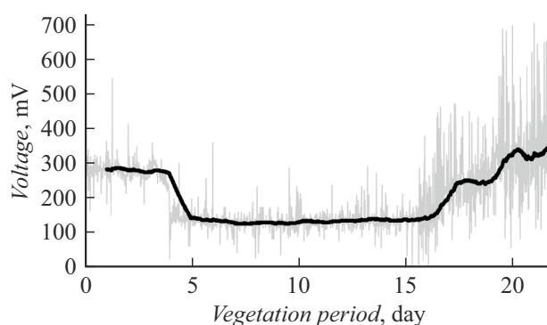
Figure 3. Dynamics of potential difference formation in three BES cells connected in series during cultivation of lettuce plants.
