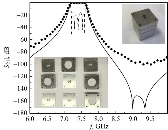
Figure 3. Amplitude-frequency response of the synthesized filter, experimental data (markers) and photos of the created filter assembly and component.
