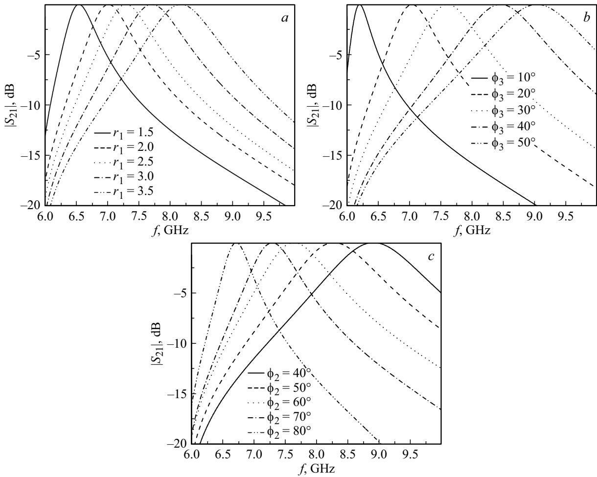
Figure 2. Transmission Ratio Module vs. Frequency and Aperture Size.
