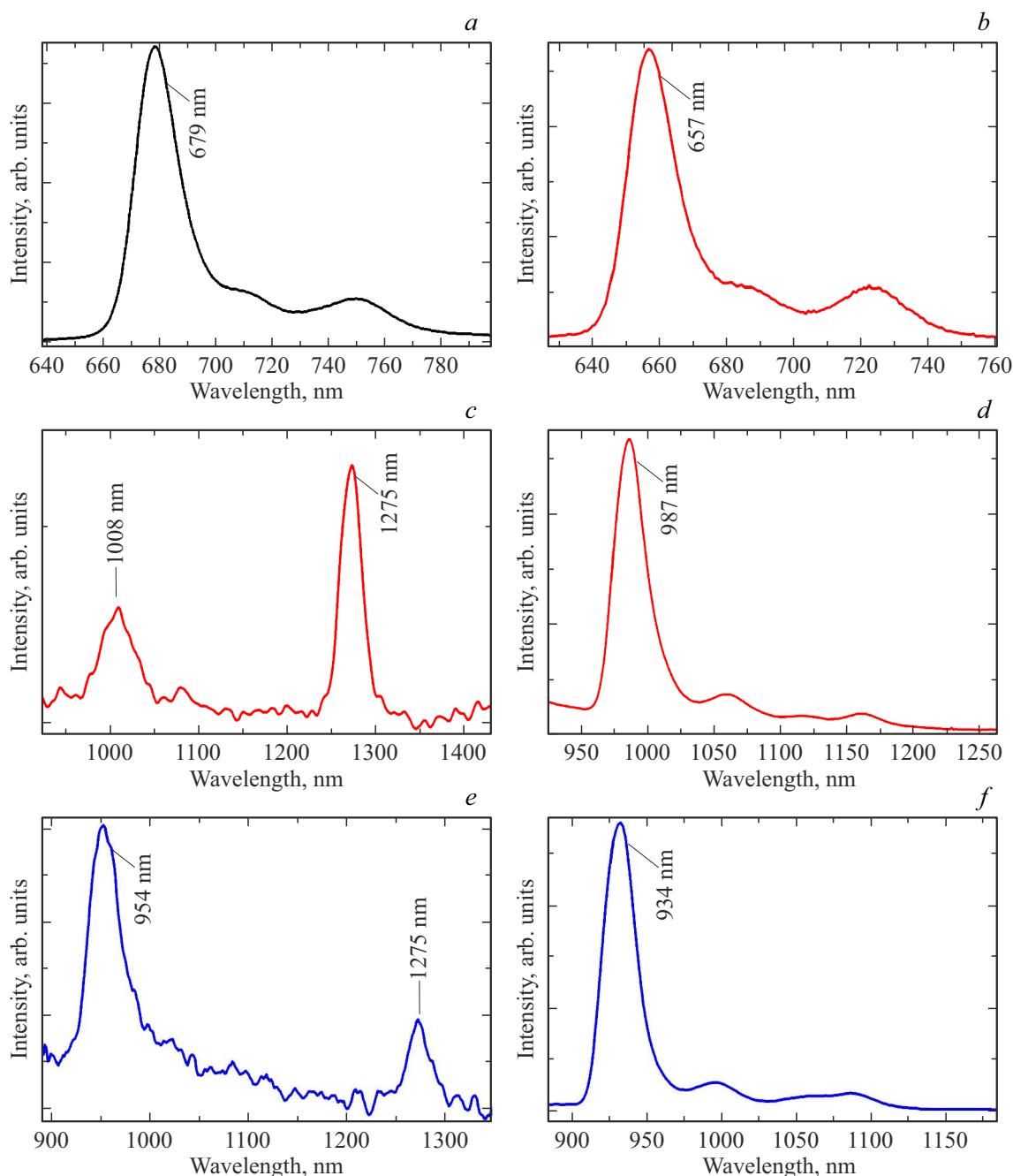
Figure 3. Fluorescence spectra of Mg-Pc (a) and Pd-Pc (b), phosphorescence spectra of Pd-Pc (c) and Pt-Pc (e) at 293 K phosphorescence spectra of Pd-Pc (d) and Pt-Pc (f) at 77 K in toluene and \lambda_{\text{exc}} = 340 nm.
