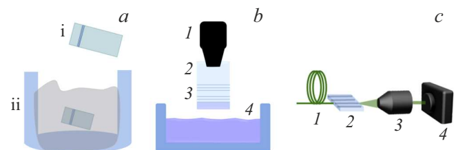
Figure 3. Schematic flow diagram of the test of created optofluidic elements: (a) two stages of microchannels formation: (i) — writing of tracks in the NPSM material decompaction mode, and (ii) — cleaning of the decompaction tracks in water from the debris; (b) study of permeability of barriers: 1 — holder, 2 — NPSM, 3 — barriers in NPSM, 4 — pigment solution; (c) introduction of radiation into waveguides: 1 — optic fiber, 2 — NPSM with channel waveguides, 3 — objective (40x, NA 0.65), 4 — CMOS camera Gentec 3M.
