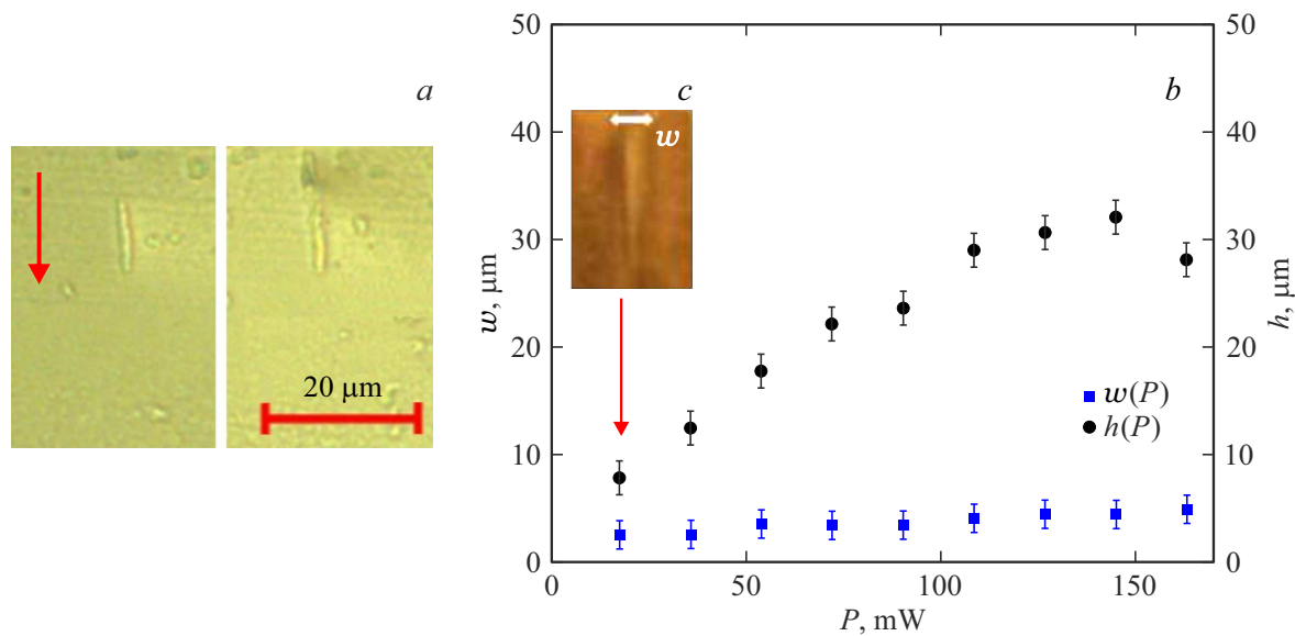
Figure 6. (a) Microphotographs of asymmetric waveguides (end view, the arrow indicates direction of laser beam in the process of laser direct writing); (b) dependence of the width of cross-section of waveguide on the power of laser radiation; (c) cross-section of waveguide with the power of laser radiation 17–50 mW.
