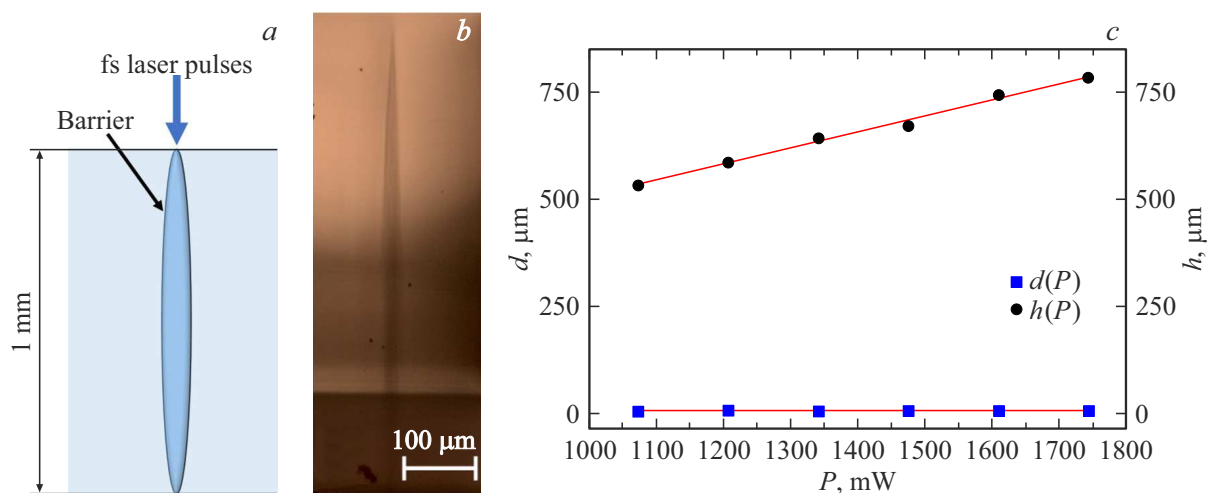
Figure 4. (a) Schematic diagram of the barrier in a NPSM plate; (b) microphotograph of the barrier recorded at the power of 1540 mW and scanning speed of 1 mm/s; (c) dependence of the barrier height ( h ) and ( d ) width in cross-section on the radiation power.
