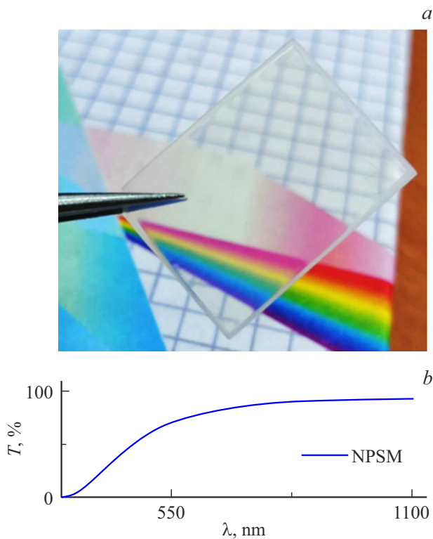
Figure 1. (a) Photo of NPSM; (b) transmission spectrum within the range of 300–1100 nm.
