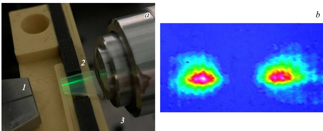
Figure 7. (a) Photograph of the process of the radiation introduction into waveguide: 1 — fiber, 2 — NPSM with a set of channel waveguides with the placement period of 10 μm and 3 — objective; (b) near-field distribution of intensity at the exit from the waveguide.
