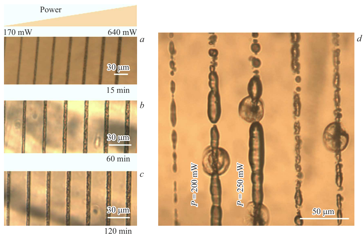
Figure 9. Microphotograph of microchannels after cleaning in distilled water under the effect of ultrasound 15 (a), 60 (b) and 120 min (c), (d) after the sample heat treatment.
