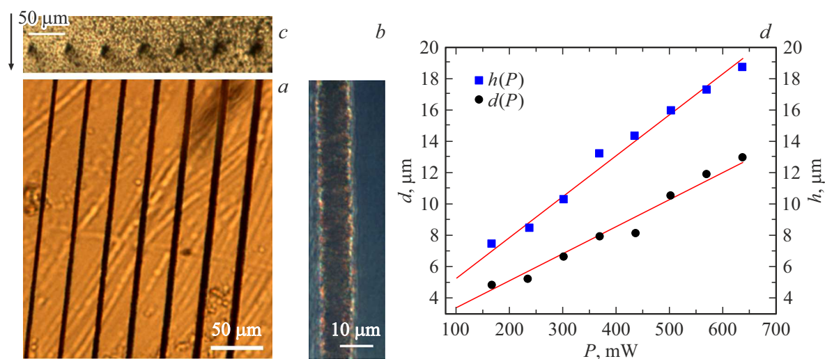
Figure 8. (a) Microphotograph of the material decompaction tracks after laser writing (c) view of the cross-section after polishing, the arrow indicates direction of laser beam in the process of writing and (b) microphotograph of the decompaction track under crossed polarizer and analyzer; (d) the graph of dependence of the diameter and height of cross-section of microchannel on the laser power.
