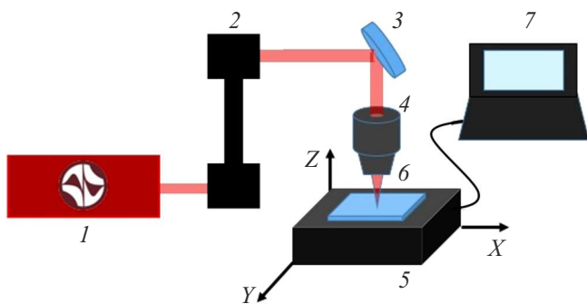
Figure 2. Diagram of experimental setup for direct laser writing: femtosecond laser (1), periscope (2), dielectric mirrors (3), objective (4), three-coordinate system (5), sample (6), PC (7).
