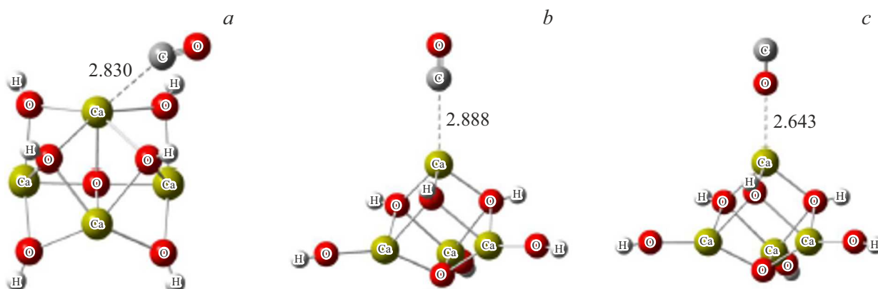
Figure 3. Modification of cluster \text{Ca}_4\text{O}_4 by molecules \text{H}_2\text{O} . See details in the text.
