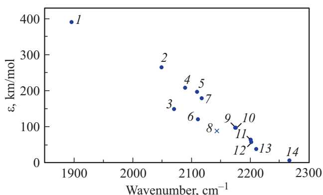
Figure 6. Correlation between the calculated values of frequency and intensity of the vibration stripe of C–O in the studied complexes. 1 — \text{Ca}^{2+} + \text{OC} , 2 — \text{CaAl}(\text{OH})_4 + \text{OC} , 3 — \text{Ca}_4\text{O}_4 + 3\text{SO}_3 + \text{OC} , 4 — \text{Ca}_4\text{O}_4 + 3\text{H}_2\text{O} + \text{OC} , 5 — \text{Ca}_4\text{O}_4 + 3\text{SO}_2 + \text{OC} , 6 — \text{Ca}_4\text{O}_4 + 3\text{CO}_2 + \text{OC} , 7 — \text{Ca}_4\text{O}_4 + \text{OC} , 8 — \text{CO} , 9 — \text{Ca}_4\text{O}_4 + 3\text{CO}_2 + \text{CO} , 10 — \text{Ca}_4\text{O}_4 + 3\text{SO}_2 + \text{CO} , 11 — \text{Ca}_4\text{O}_4 + 3\text{H}_2\text{O} + \text{CO} , 12 — \text{Ca}_4\text{O}_4 + 3\text{SO}_3 + \text{CO} , 13 — \text{CaY} + \text{CO} , 14 — \text{Ca}^{2+} + \text{CO} .
