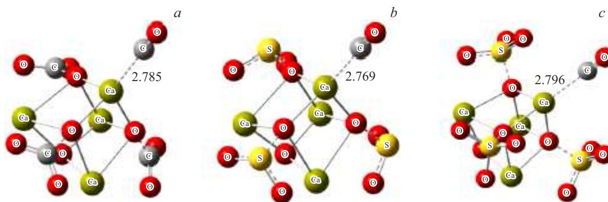
Figure 4. Modification of cluster \text{Ca}_4\text{O}_4 by molecules \text{CO}_2 (a), \text{SO}_2 (b) and \text{SO}_3 (c). See details in the text.
