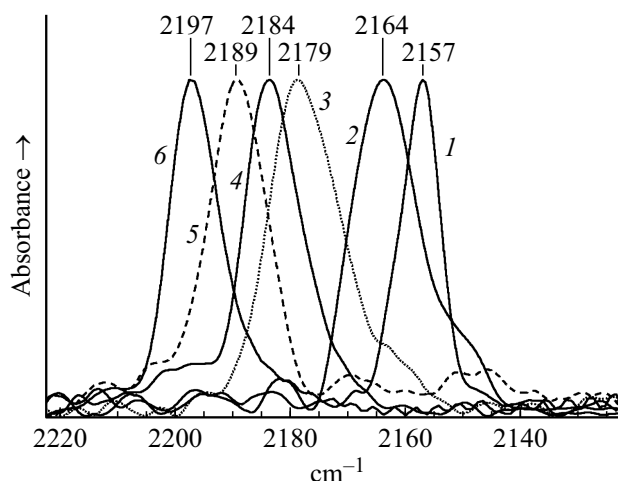
Figure 1. IR spectrum of CO adsorbed on the CaO sample thermally vacuumed at 700^\circ\text{C} and modified by adsorption of \text{H}_2\text{O} (with subsequent pumping out at 20^\circ\text{C} (1) and 500^\circ\text{C} (2)) and adsorption of \text{CO}_2 (3), \text{SO}_2 (4) and \text{SO}_3 (5). 6 — spectrum of CO adsorbed on CaY zeolite. The spectra were recorded at 77\text{ K} and rated by the temperature.
