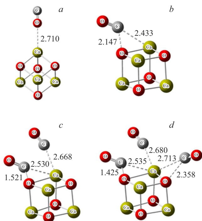
Figure 2. Interaction of the cluster \text{Ca}_4\text{O}_4 with molecules of CO. Explanations — in the text.
