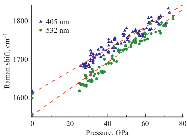
Figure 4. Dependence of the Raman frequency of 3D C_{60} on pressure. Spectra were measured at a laser power of 15 mW, the measurement time was 10 min, and the excitation radiation wavelengths were 405 nm (triangles) and 532 nm (circles).
