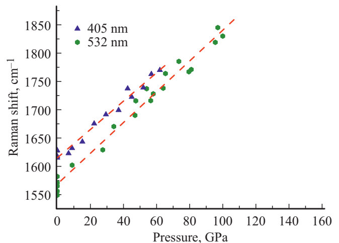
Figure 3. Dependence of the Raman frequency of 3D \text{C}_{60} on pressure. Spectra were measured at a laser power of 1 mW, the measurement time was 10 min, and the excitation radiation wavelengths were 405 nm (triangles) and 532 nm (circles). The presented data cover the interval from the phase formation under 25 GPa to a pressure of 101 GPa under which the spectrum of 3D \text{C}_{60} was still observed.
