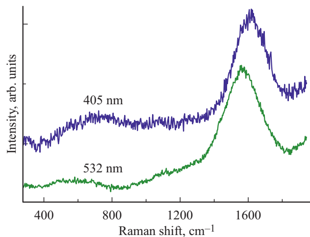
Figure 2. Raman spectra of the 3D \text{C}_{60} sample. Spectra obtained prior to unloading were measured at a laser power of 1 mW. The measurement time was 10 min, and the excitation radiation wavelengths were 405 and 532 nm.
