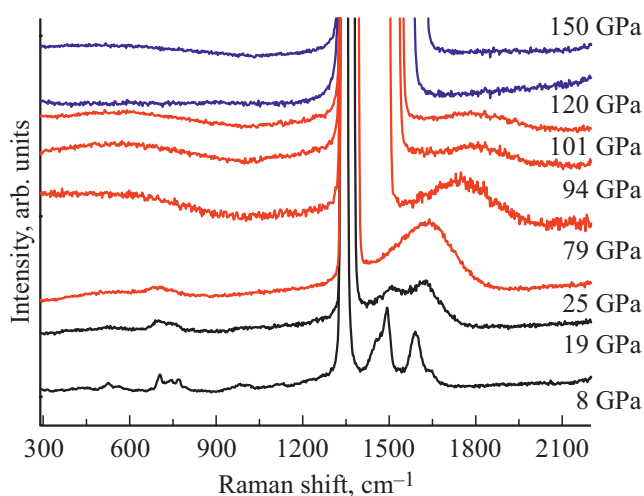
Figure 1. Pressure-induced transformation of Raman spectra of fullerene \text{C}_{60} .
