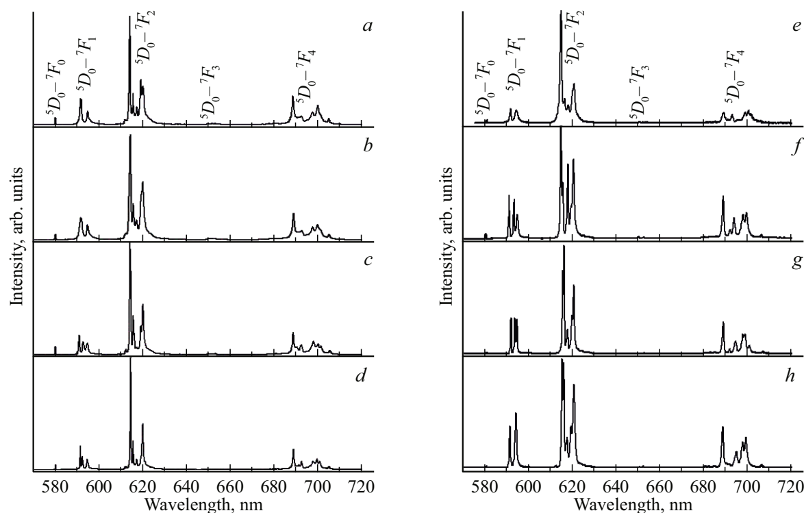
Рис. 3. Спектры люминесценции соединений [\text{Eu}_2(\text{Piv})_6(\text{DMPhen})_2] (2) (a), [\text{Eu}_2(\text{Piv})_6(\text{MPhen})_2] (3) (b), [\text{Eu}_2(\text{Piv})_6(\text{APhen})_2] (4) (c), [\text{Eu}_2(\text{Piv})_6(\text{Phen})_2] (5) (d), [\text{Eu}_2(4\text{-MOBA})_6(\text{Bpy})_2] (1) (e), [\text{Eu}_2(\text{Capr})_6(\text{Phen})_2] (6) (f), [\text{Eu}_2(\text{Ac})_6(\text{Phen})_2] (7) (g), [\text{Eu}_2(\text{Prop})_6(\text{Phen})_2] (8) (h) при 77 К.
