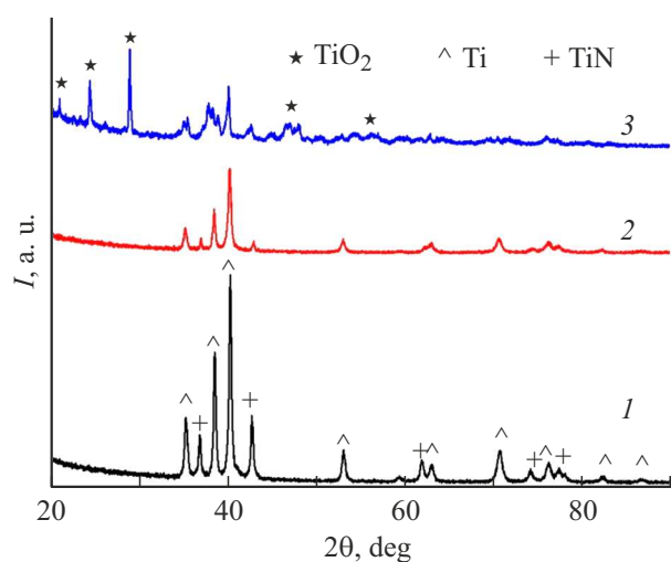
Figure 4. Diffraction patterns of Ti + 50 wt.% TiN (mixture 2). 1 — sputtering powder, 2 — CS-coating before heat treatment, 3 — after heat treatment.
