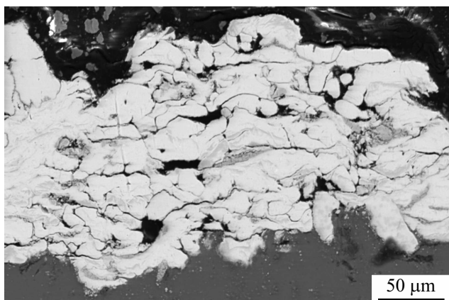
Figure 3. Micrograph of a cross-section of CS coatings after high-temperature treatment of Ti + 50 wt.% TiN composition (mixture 3).
