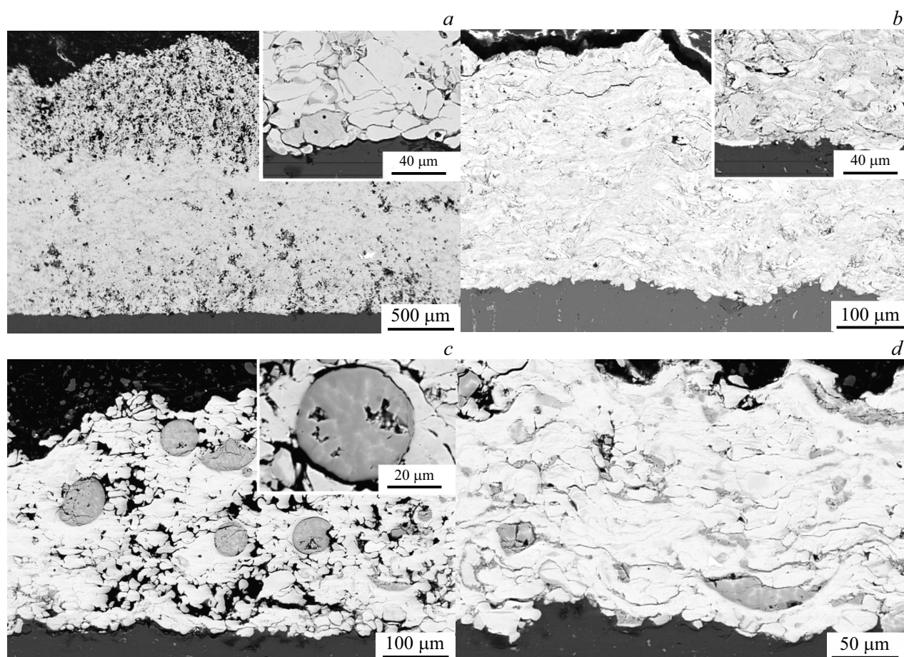
Figure 2. Micrographs of the cross-section of CS-coatings of various composition. a — titanium, b — Ti + 25 wt.% TiN (mixture 1), c — Ti + 50 wt.% TiN (mixture 2), d — Ti + 50 wt.% TiN (mixture 3).
