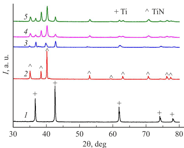
Figure 1. X-ray diffraction patterns of initial (1, 2), spheroidized (3) and machined (4, 5) particles of titanium (1), titanium nitride (2, 3), mixture of Ti + 25 wt.% TiN (4), mixture of Ti + 50 wt.% TiN (5).
