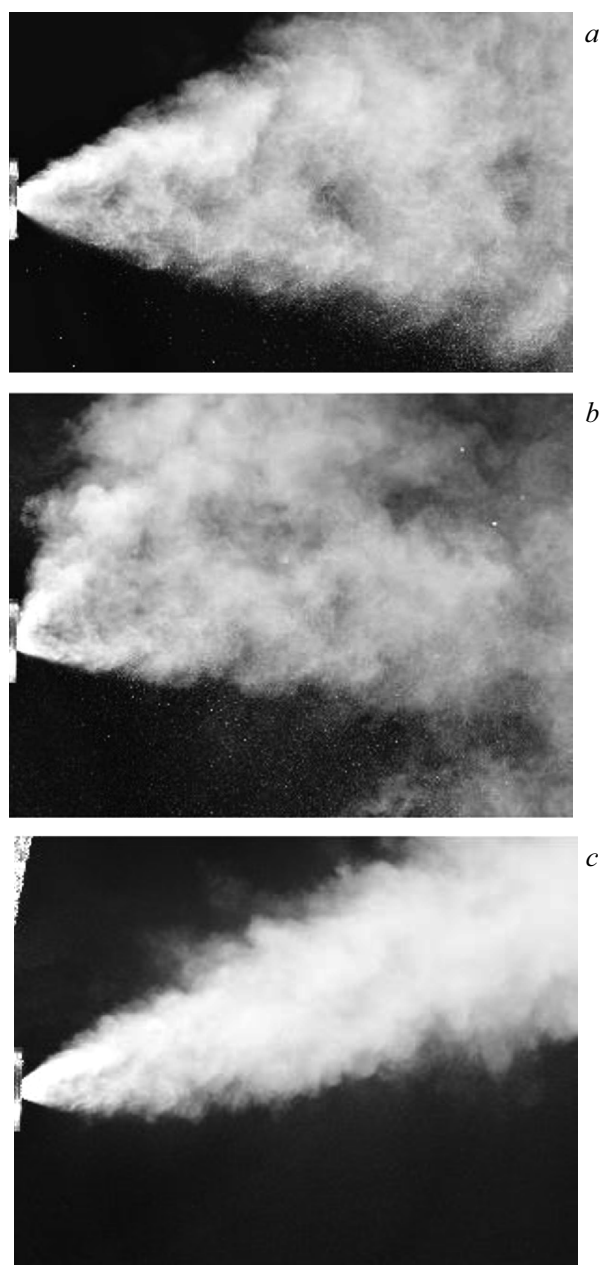
Figure 3. Jets of superheated water at different high temperatures: T_s = 180 (a), 210 (b) and 310 °C (c).
