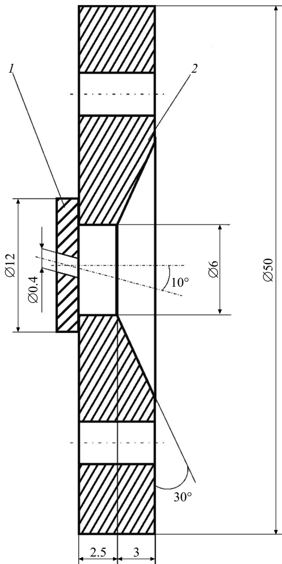
Figure 1. Cut of a short cylindrical nozzle (1) and a clamping flange (2) with cylindrical and diffusion parts.
