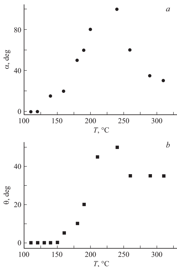
Figure 4. Temperature dependence of the opening angle (a) and the deflection angle (b) of a boiling-up liquid jet.
