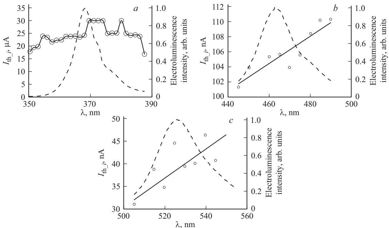
Figure 3. Dependence of the threshold current on the wavelength of the emission spectrum of ultraviolet (a), blue (b) and green (c) LED. Dashed lines specify the emission spectra of LED.
