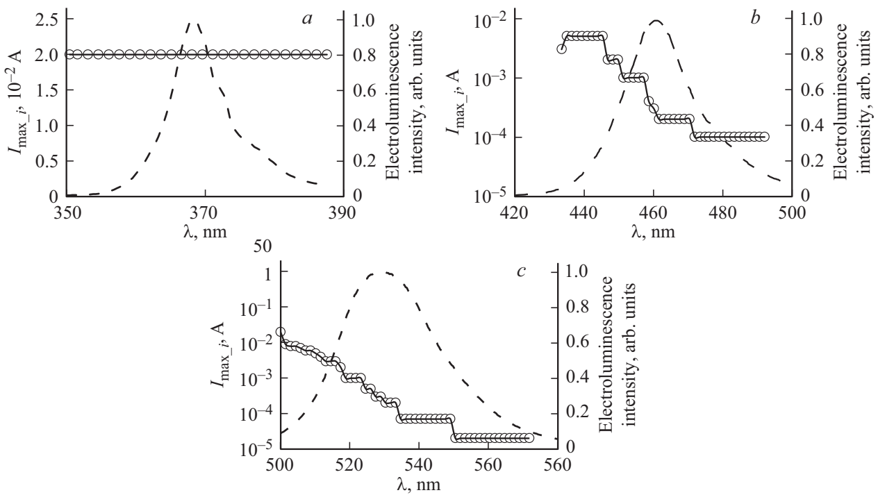
Figure 2. Current dependence, at which the maximum IQE is reached, being measured in different parts of the spectrum, on the wavelength of the ultraviolet (a), blue (b) and green (c) LED. Dashed lines specify the emission spectra of LED.
