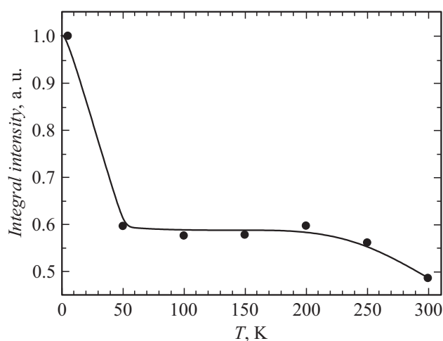
Figure 2. Temperature dependence of integral intensity of PL band of \text{Gd}^{3+} ions in preform for optical fibers. Excitation wavelength is 150 nm.
