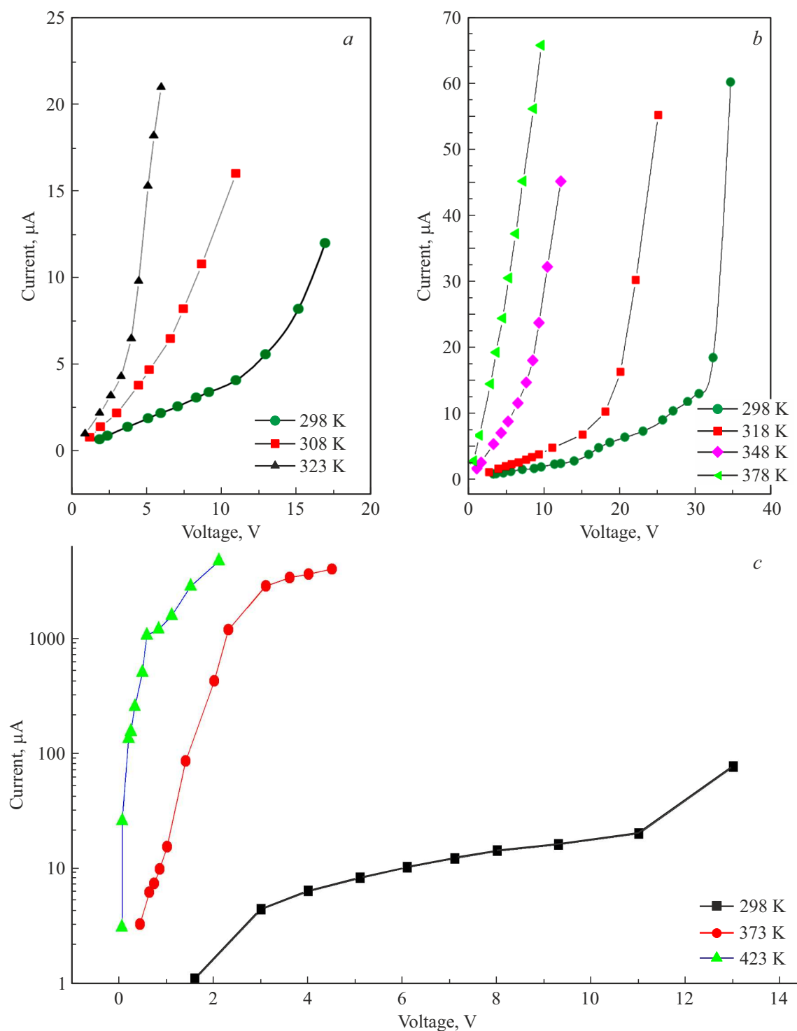
Figure 6. VACs for plates made of crystals of the AgBr–AgI systems: (a) \text{AgBr}_{0.76}\text{I}_{0.24} 0.5 mm thick, (b) \text{AgBr}_{0.76}\text{I}_{0.24} thickness 1.7 mm, (c) \text{AgBr}_{0.96}\text{I}_{0.04} 0.5 mm thick, at various temperatures.
