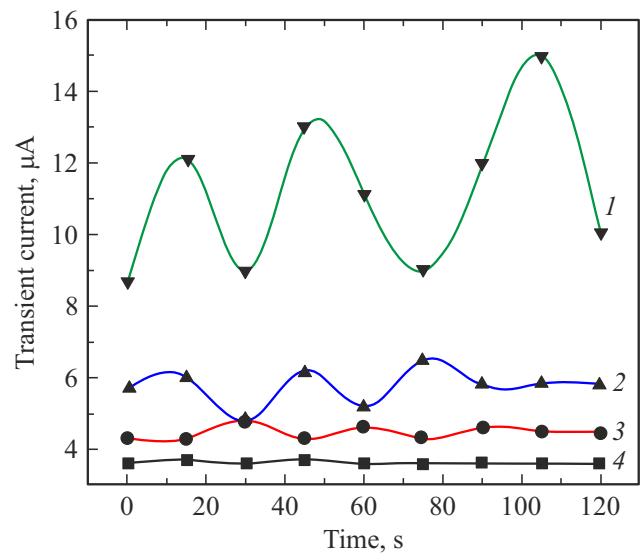
Figure 10. Transient characteristics of the current at a step voltage on a 0.5 mm thick \text{AgBr}_{0.96}\text{I}_{0.04} plate at a temperature of 298 K: 1 — 8.7 V; 2 — 5.7 V; 3 — 4.3 V; 4 — 3.6 V.
